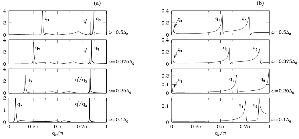
FIG. 11: |Im\Lambda(q, \omega)/\pi| versus q for a d -wave superconductor with a tight-binding band given by Eq. (28) with t'/t = -0.3 , \mu/t = -1.0 , \Delta_0 = 0.1t . Here (a) shows results for a diagonal cut for q_x = q_y and (b) shows results for a horizontal q_y = 0 cut. The q_\alpha and q' vectors are shown in Fig 10(a).
